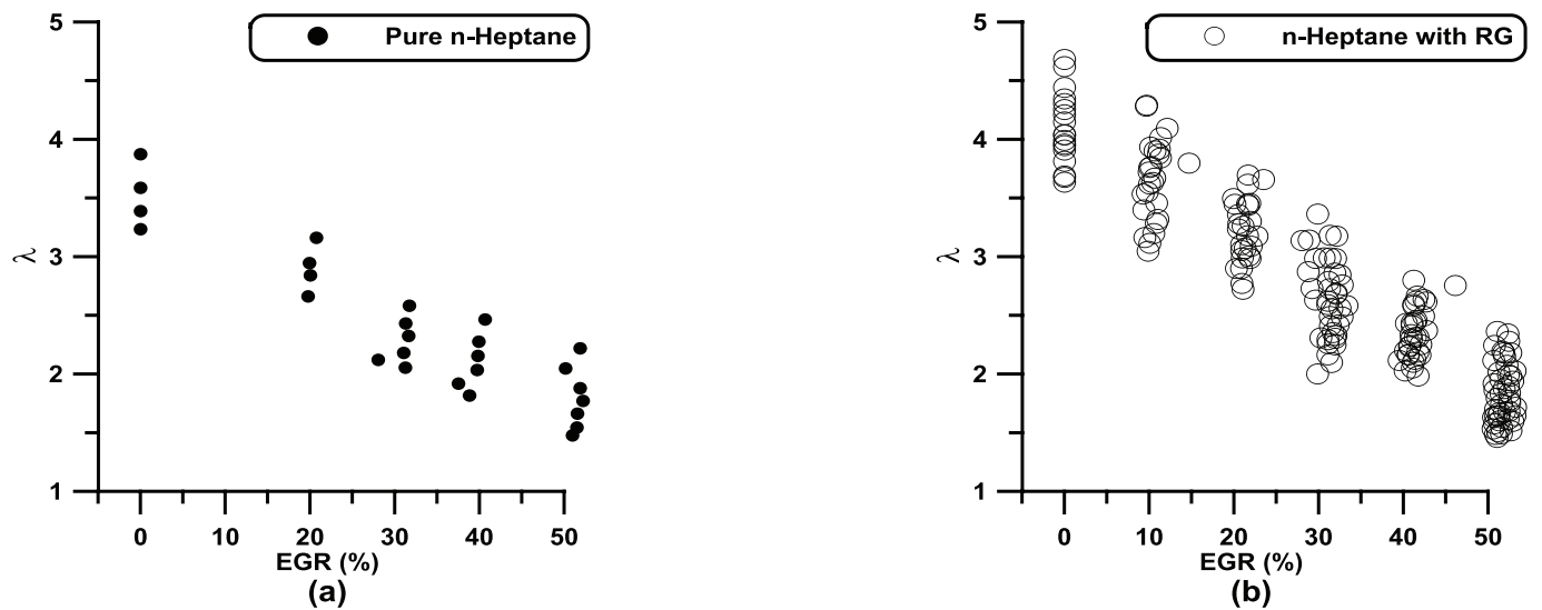
Fig. 13. \lambda -EGR operating region of n-Heptane HCCI combustion (a) pure n-Heptane and (b) n-Heptane enriched with RG
